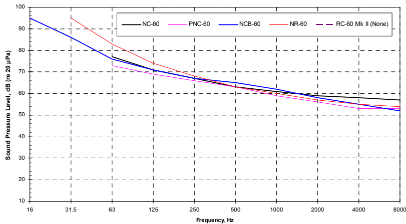
Comparison of Perception-based Criterion Curves ("Noisy" Labs, e.g., cleanrooms)
