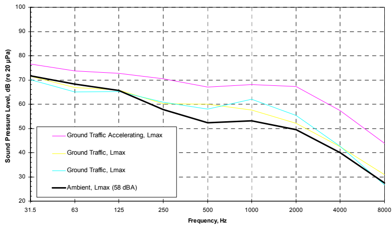
Sound Pressure Levels of Automobile Traffic (noisy urban environment - 300m from roadway at building facade)
