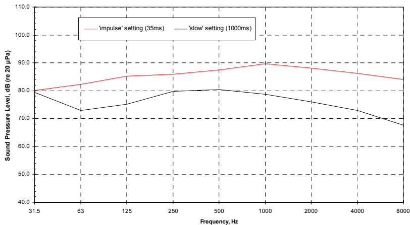
Effect of Time Constant on Measured Amplitude ("Packaging Machine" - Impulsive Noise)
