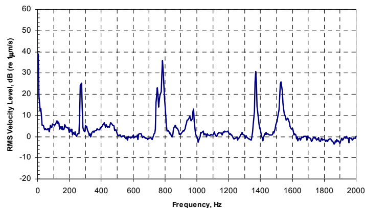
Noise induced vibration in a 210 x 350 x 6 mm thick aluminum plate (Source: white noise)
