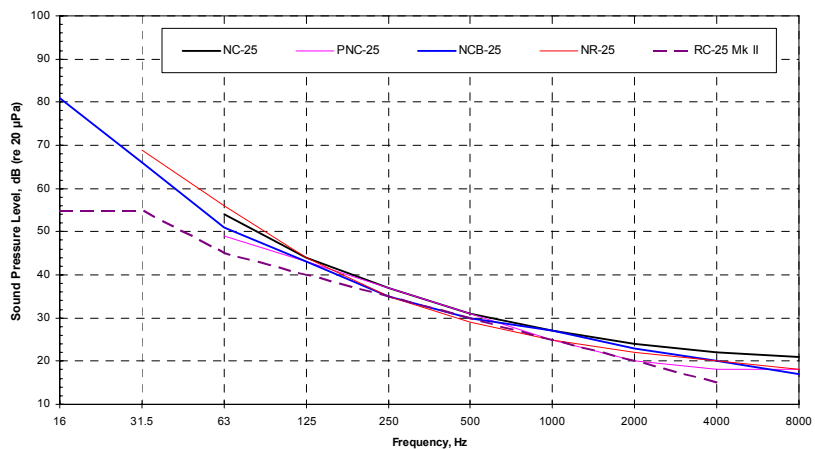
Comparison of Perception-based Criterion Curves ("Quiet" Labs)
