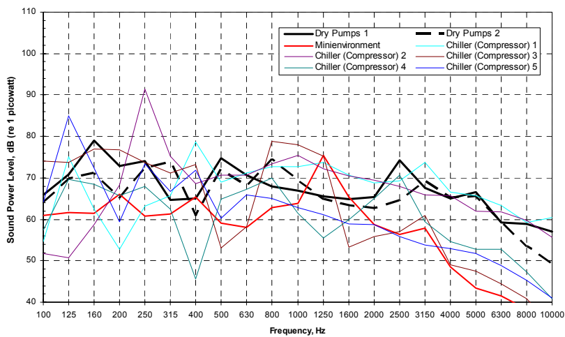
Sound Power Levels of Various Advanced Technology Tool Support Equipment
