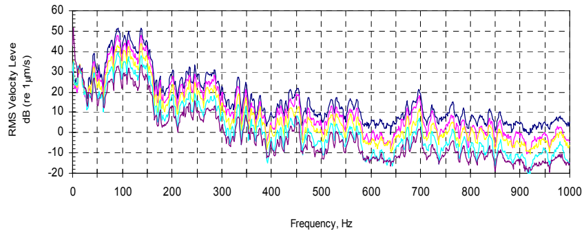
Noise induced vibration in a 560 x 710 x 0.4 mm thick steel panel (Source: white noise at 5 different amplitudes)
