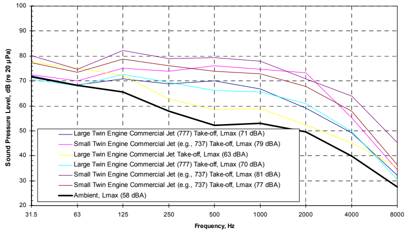
Sound Pressure Levels of Contemporary Commercial Jet Aircraft (noisy urban environment - 1 km from airport in flight path)
